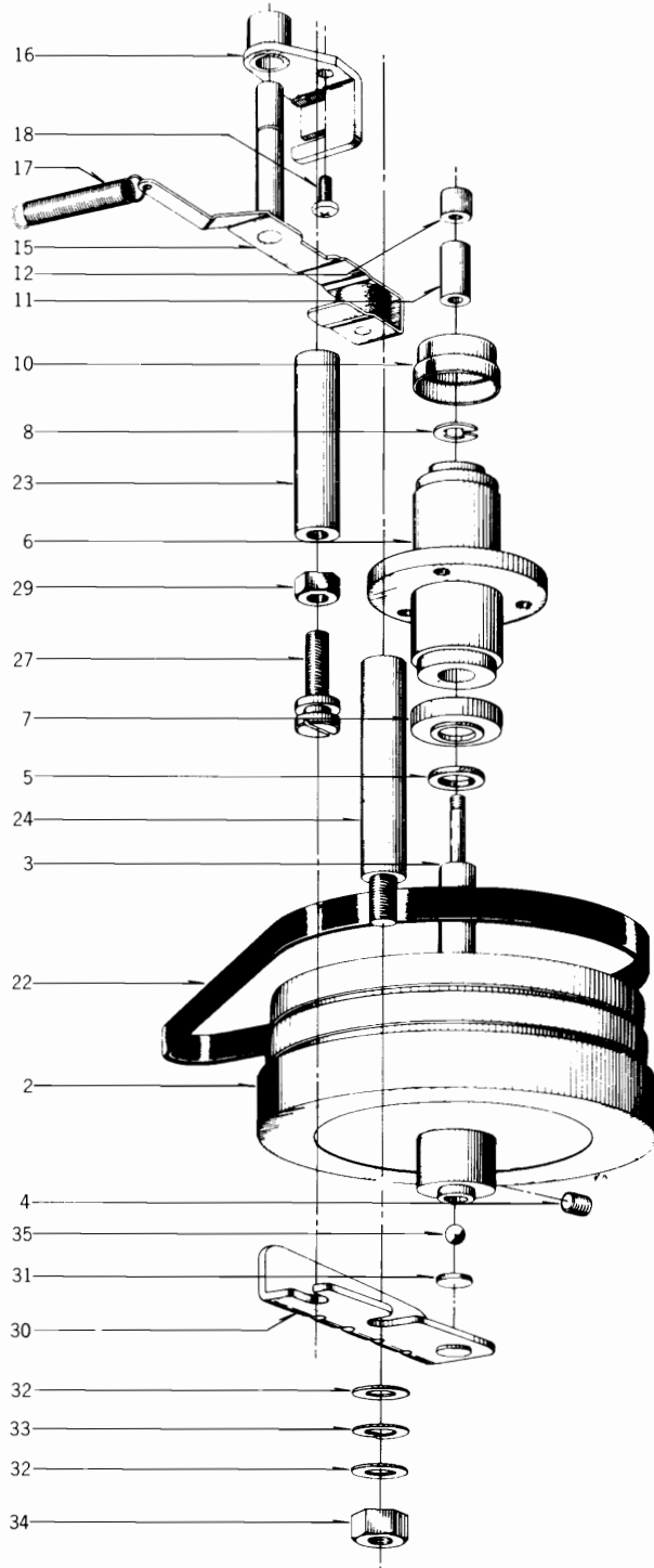
FIG. 4 ILLUSTRATION OF FLYWHEEL/ BELT CHANGE LEVER BLOCK
