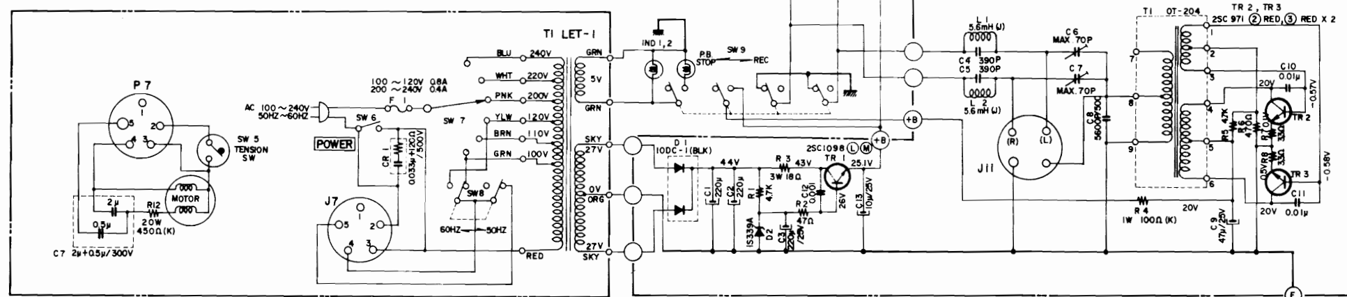
POWER SUPPLY & O.S.C. PC. BOARD. LE-5021
