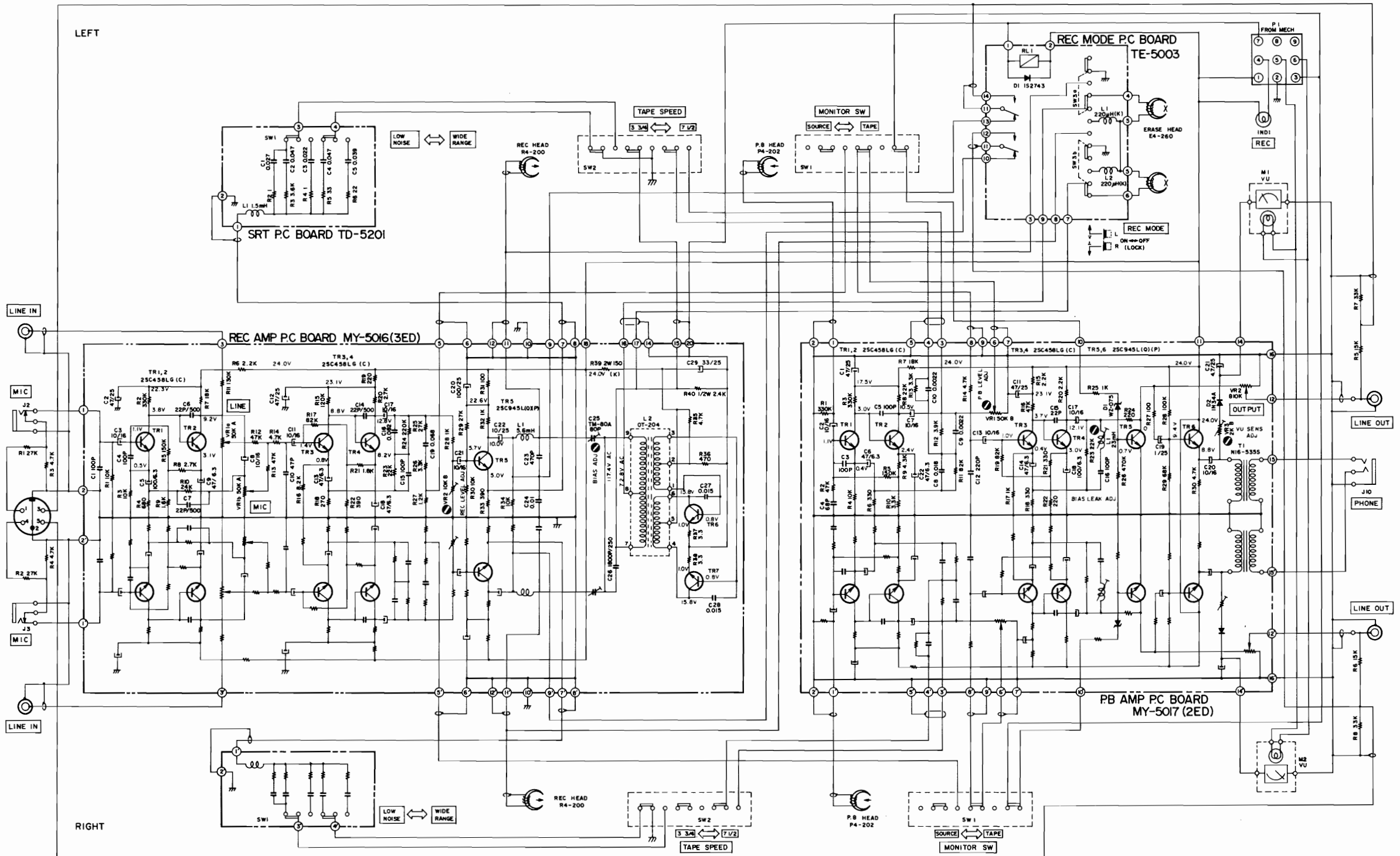
GX-630D SCHEMATIC DIAGRAM No. 5-1 1501636A
