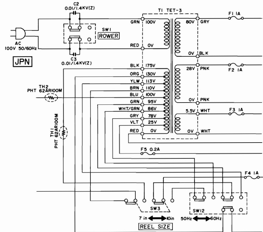
GX-630D/DB SCHEMATIC DIAGRAM No. 5-5 1501640A
